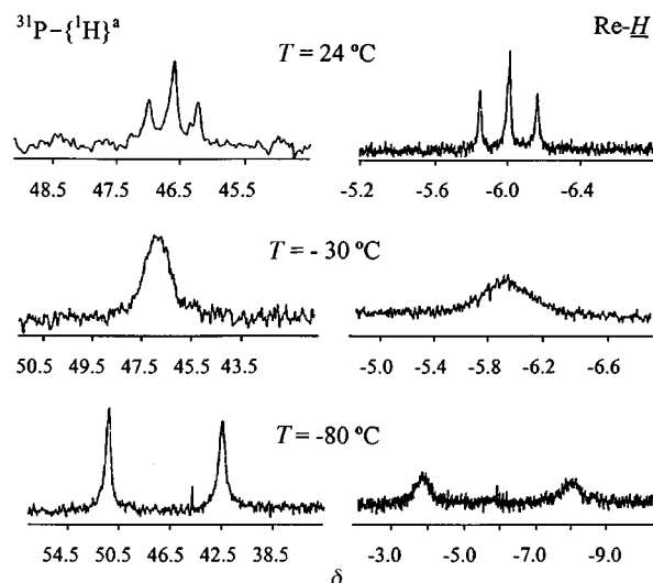
Fig. 1 Variable temperature ^1\text{H} (in the \text{ReH} region) and ^{31}\text{P} NMR spectra for complex 1 . a At 24 °C the ^{31}\text{P} NMR spectrum is the ^{31}\text{P}\{^1\text{H}\text{ selective}\} one.
