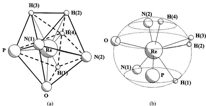
Fig. 6 Normalized co-ordination polyhedra for complex 4.
